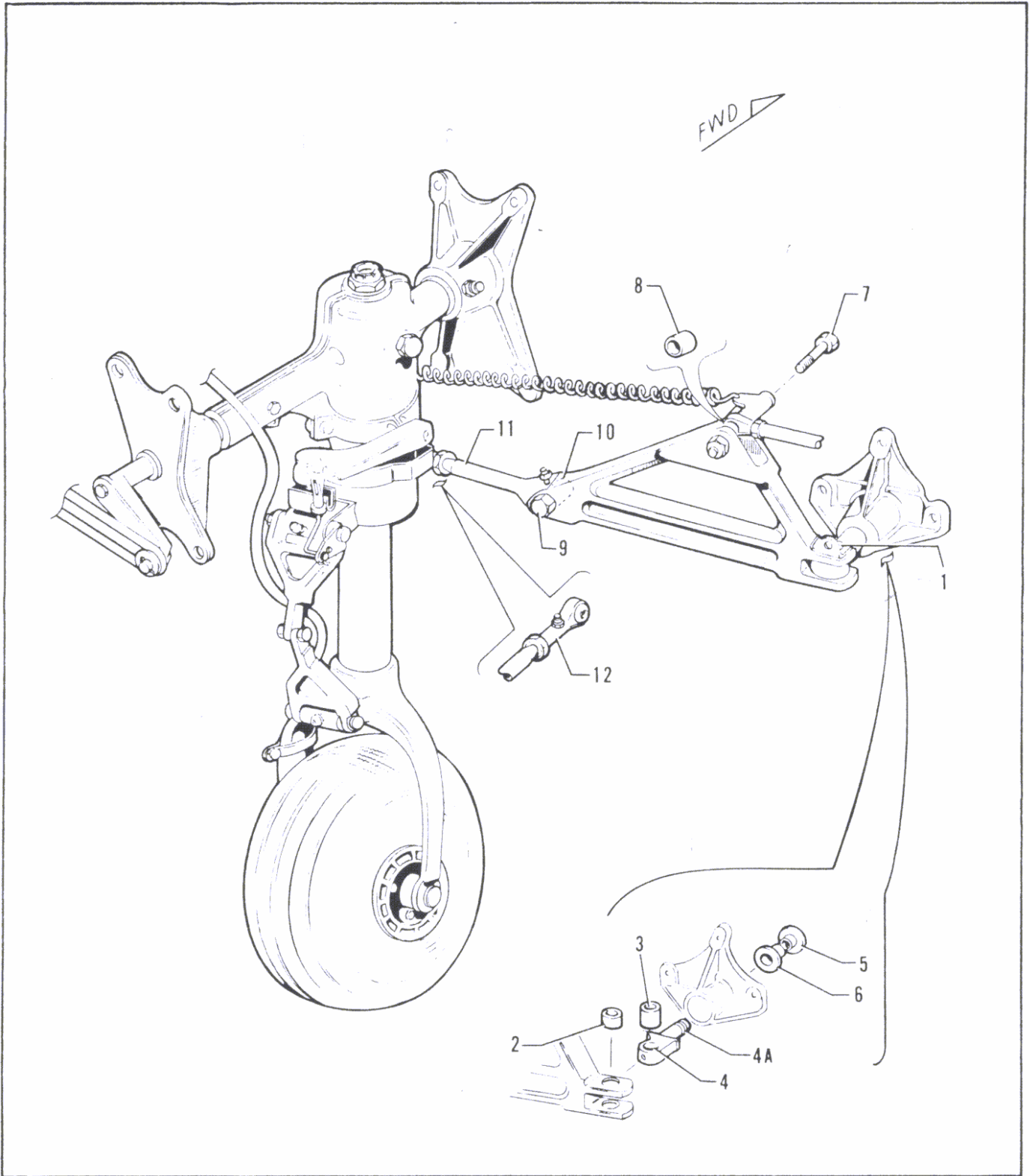
MAIN GEAR WEAR LIMITS (See Table I)
